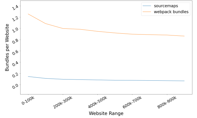
Figure 6: The prevalence of source maps
