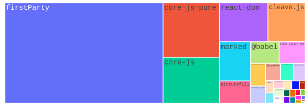
Figure 11: A transparent view of the libraries included in a bundle from readshop.nl, whose compartments are shown in Figure 10.
