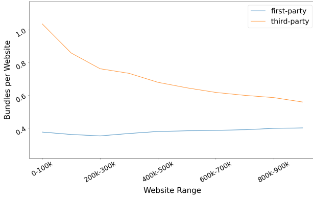
Figure 5: The origin of bundles
